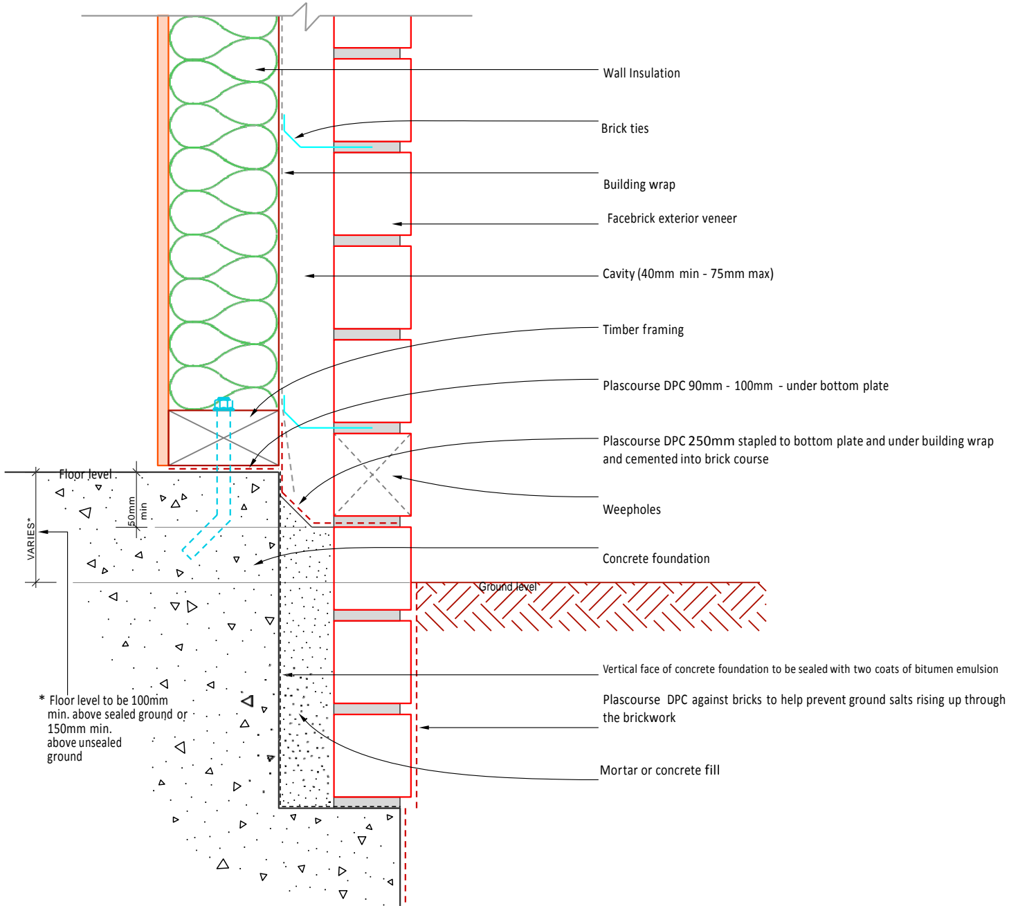
TYPICAL FOOTING DETAIL BRICK VENEER BELOW GROUND
