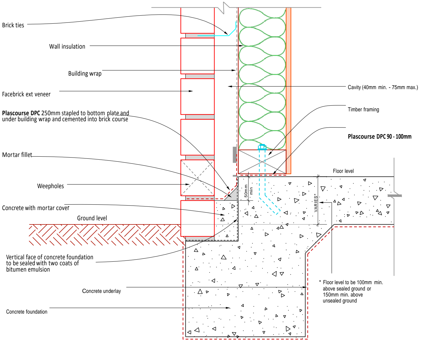
FOOTING DETAIL BRICK VENEER
